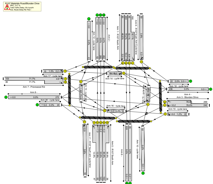
Network Layout Diagram (LinSig) - DS2028_AM
